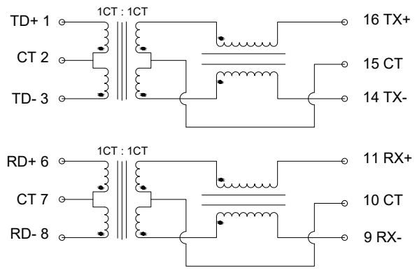
CIRCUIT SCHEMATIC
