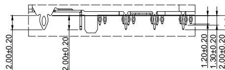
Detail A
