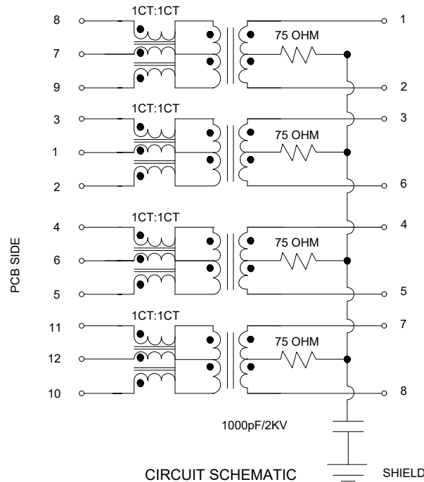
CIRCUIT SCHEMATIC
