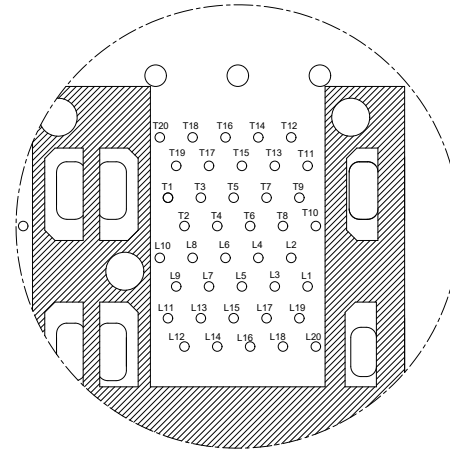
CONNECTOR PIN-OUT
