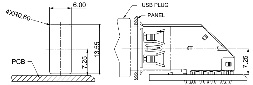
RECOMMENDED PANEL OPENING
